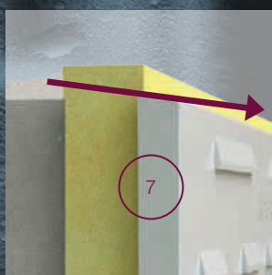
7. Edging sloped towards outer leaf to ensure wall ties sloped down.
