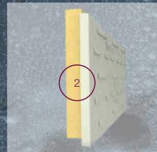
2. Engineered jointing on all edges to provide continuity of insulation layer.
